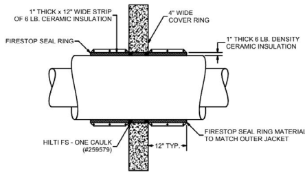
WALL PENETRATION
